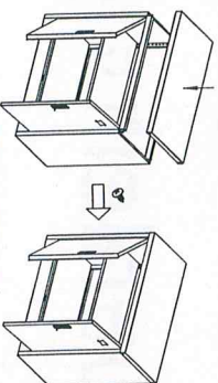
fifth installing: top board
