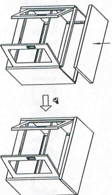
third installing: bottom board
