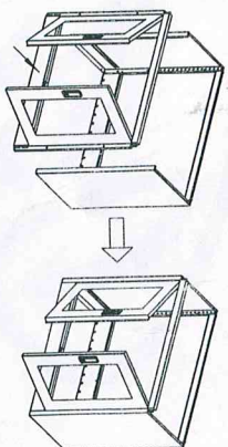
second installing: front frame
